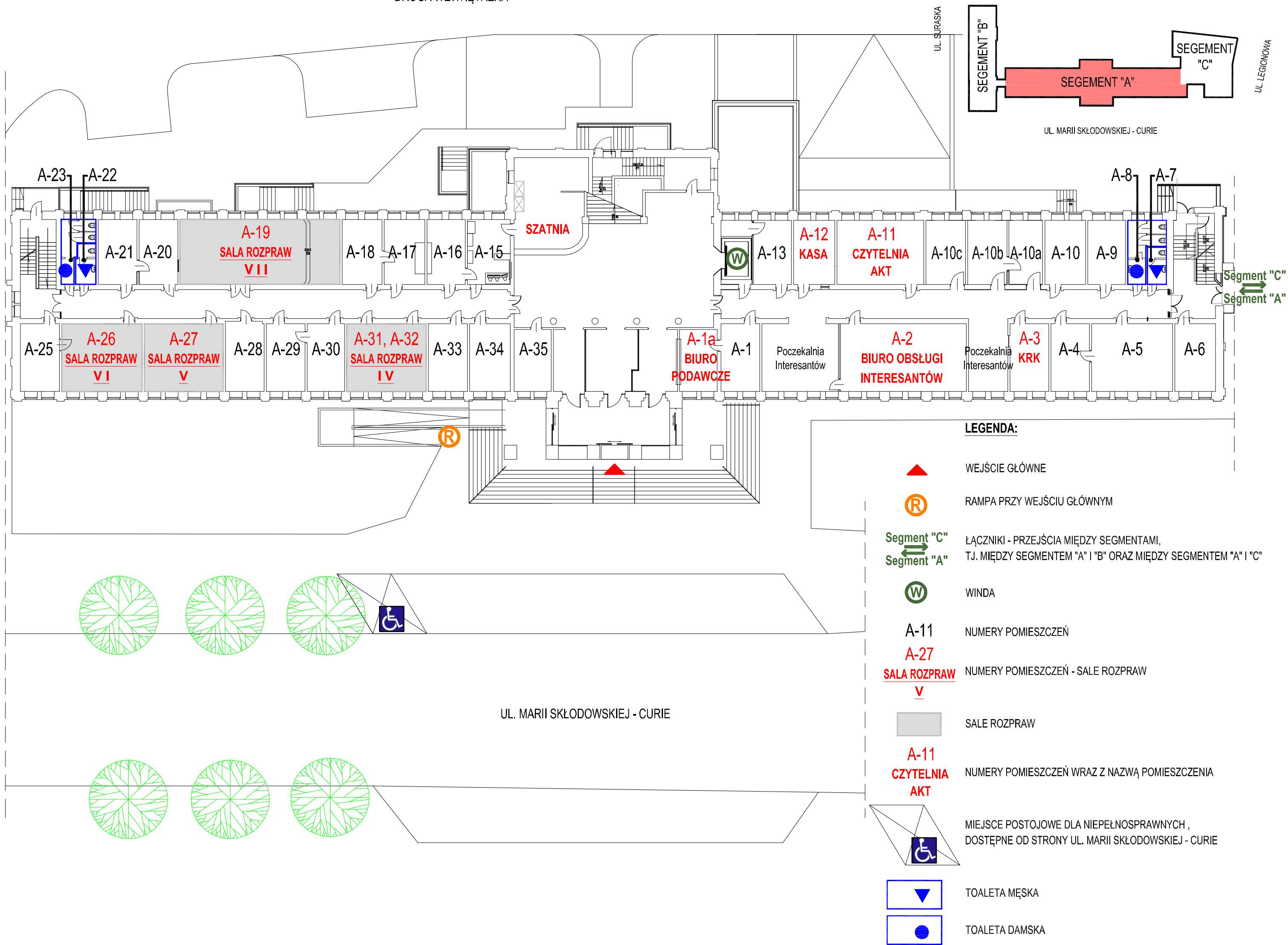
SEGMENT "A" - SCHEMAT PARTERU
